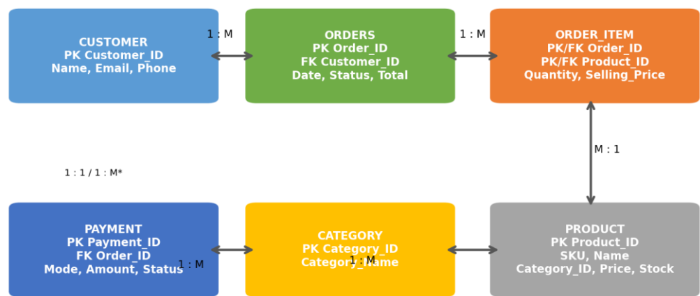
Proposed Relational ER Structure
